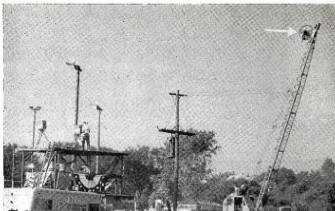
WHEN signals sent from atop a pressbox at a local softball tournament failed to reach the station's transmitter, the engineering staff of WS7D-TV Toledo mounted the microwave relay on a crane boom, ordinarily used in construction work, raising the equipment to a sufficient height of 50 feet. Then the ballgame was called on account of rain.
